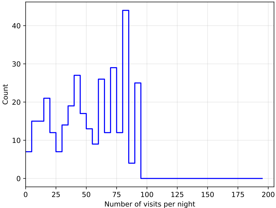
no_high_blob_v3.3_10yrs all bands: DD:EDFS NVisitsPerNight
