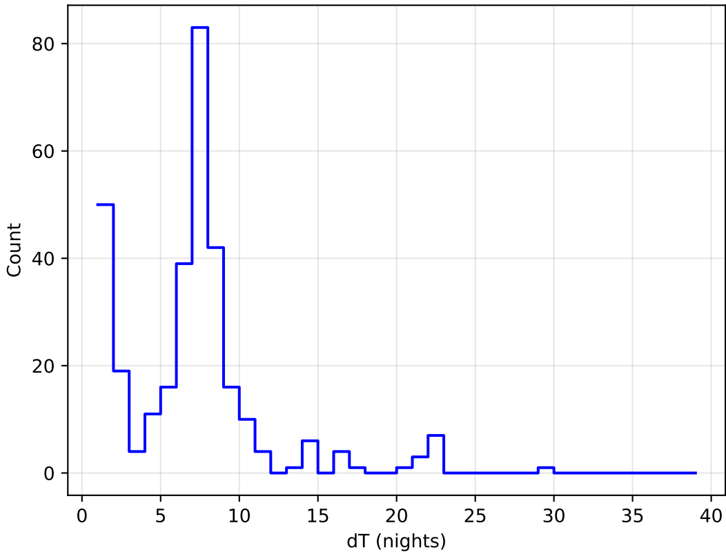
no_high_blob_v3.3_10yrs all bands: DD:EDFS Delta Nights Histogram
