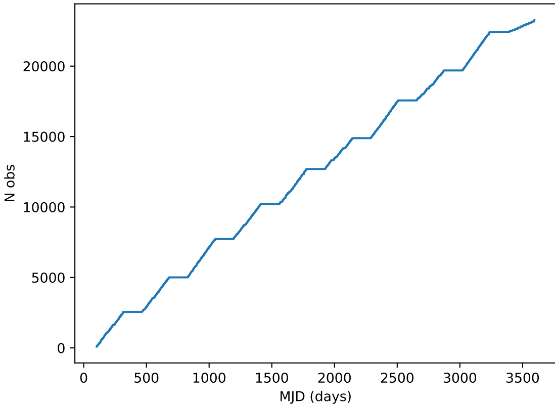
no_high_blob_v3.3_10yrs all bands: DD:EDFS Cumulative NVisits
