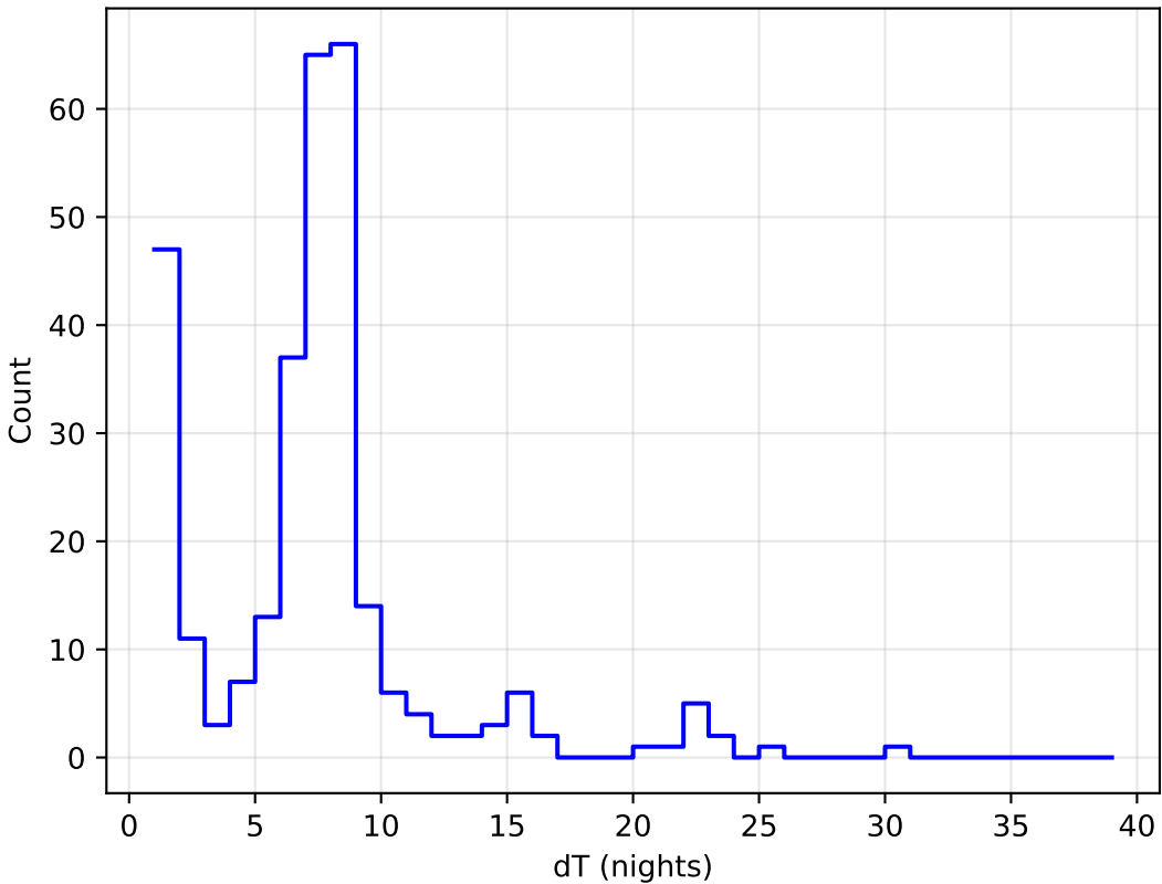
no_high_blob_v3.3_10yrs all bands: DD:ECDFS Delta Nights Histogram
