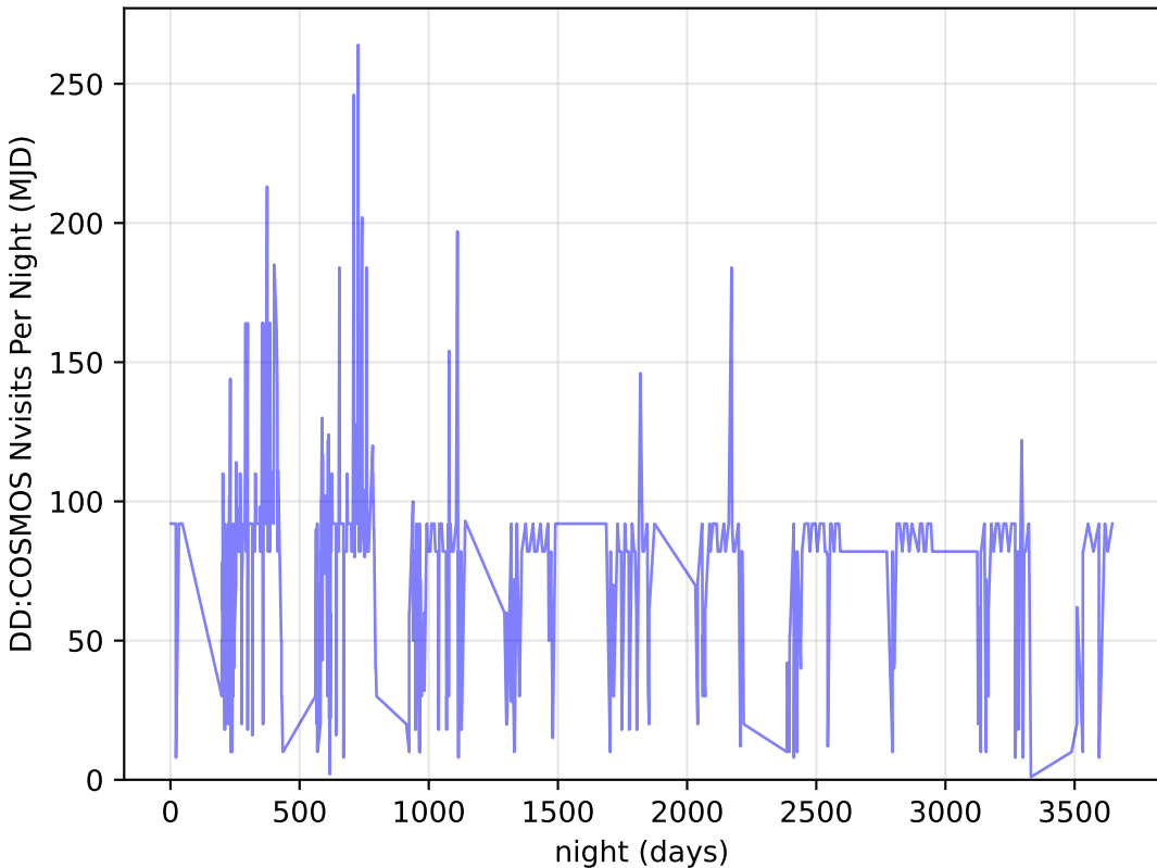
no_high_blob_v3.3_10yrs all bands: DD: COSMOS Nvisits Per Night
