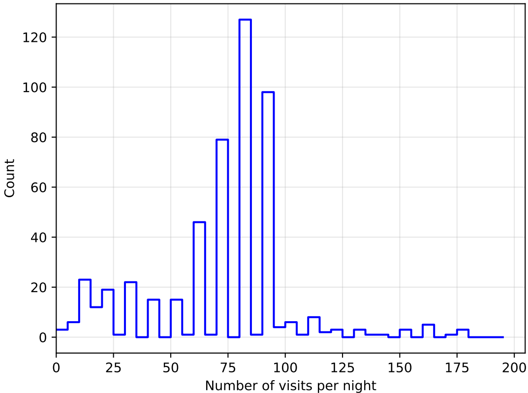
no_high_blob_v3.3_10yrs all bands: DD:COSMOS NVisitsPerNight
