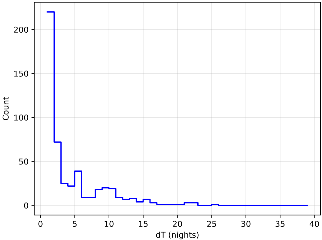
no_high_blob_v3.3_10yrs all bands: DD:COSMOS Delta Nights Histogram
