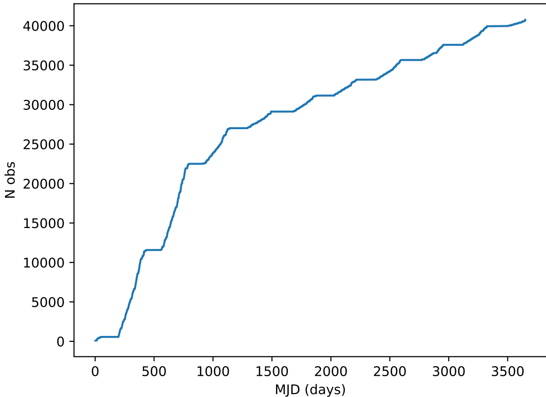
no_high_blob_v3.3_10yrs all bands: DD: COSMOS Cumulative NVisits
