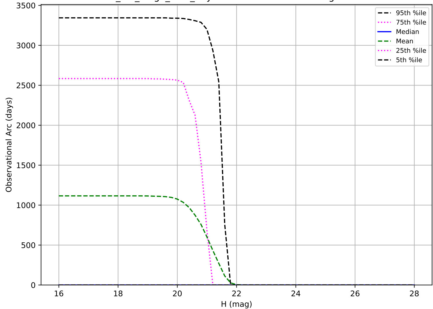
mw_roll_bulge_v3.3_10yrs: Observational Arc Length Vatira
