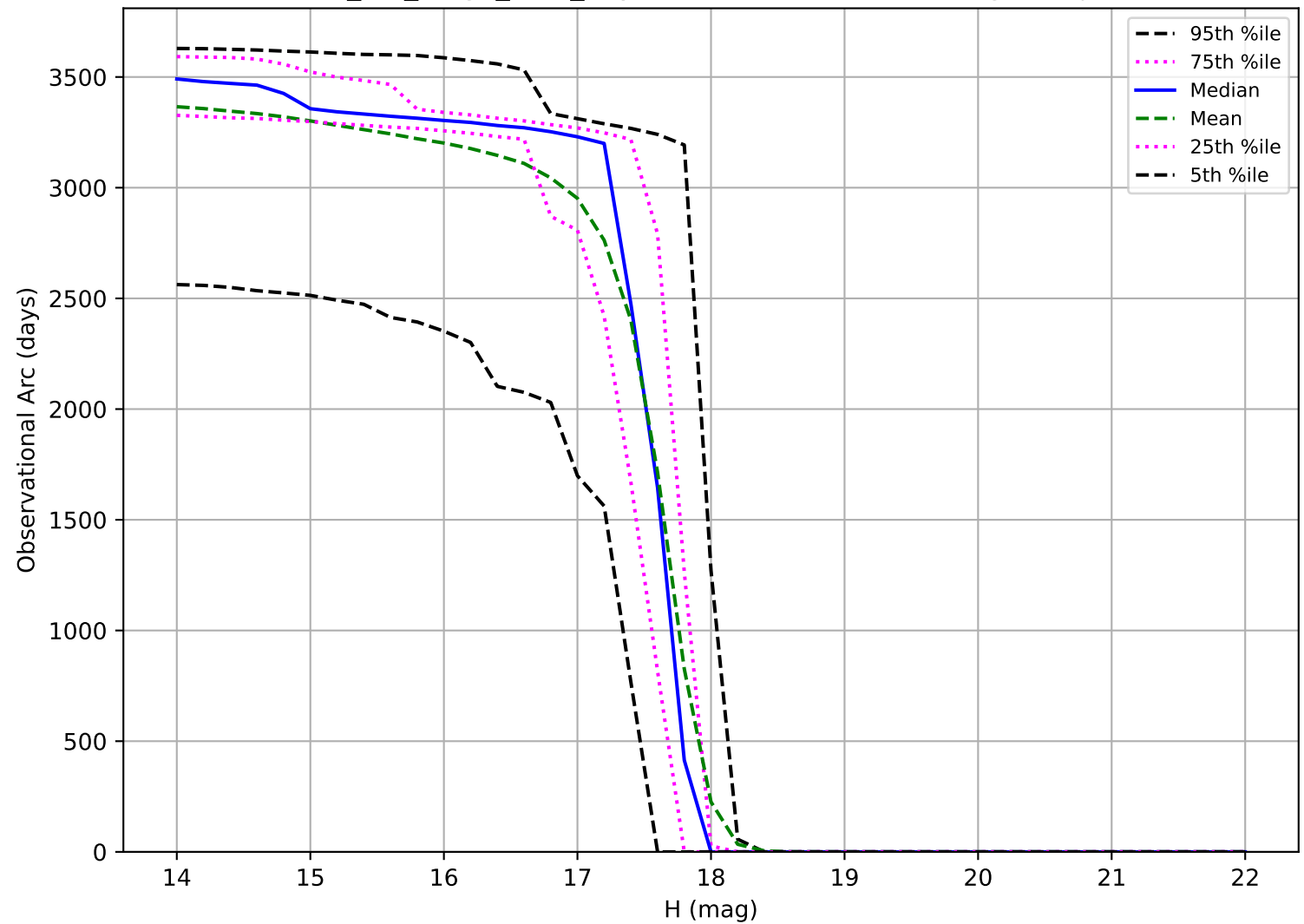
mw_roll_bulge_v3.3_10yrs: Observational Arc Length Trojan
