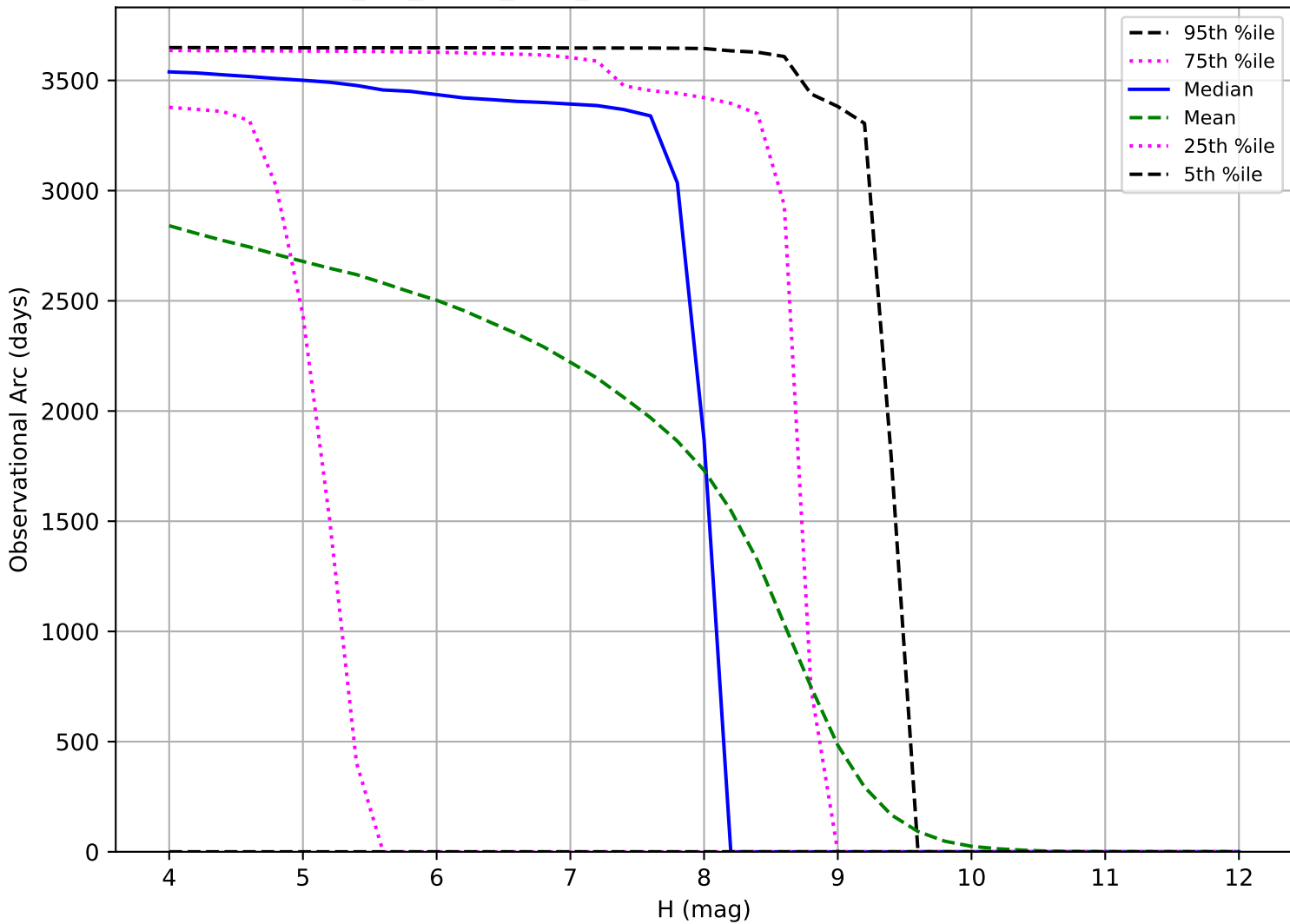
mw_roll_bulge_v3.3_10yrs: Observational Arc Length TNO
