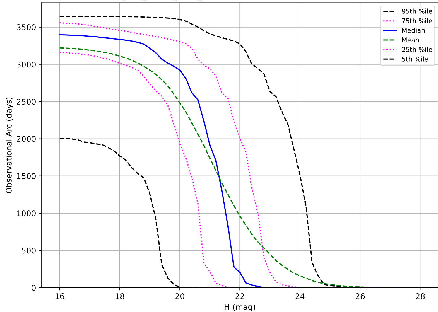
mw_roll_bulge_v3.3_10yrs: Observational Arc Length PHA
