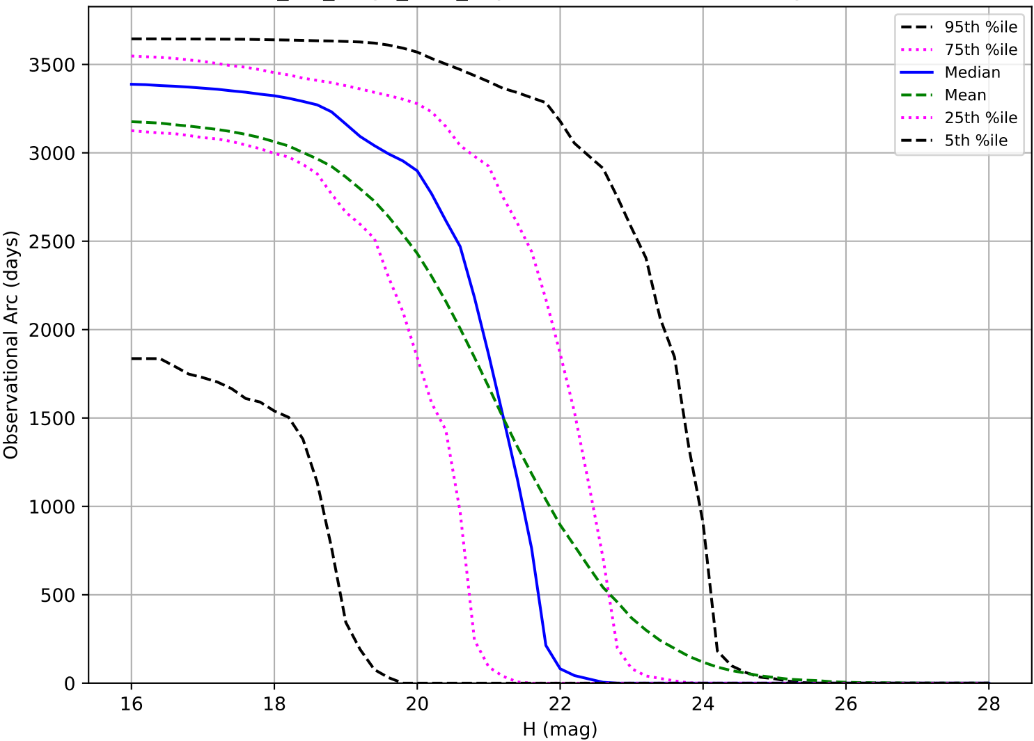
mw_roll_bulge_v3.3_10yrs: Observational Arc Length NEO
