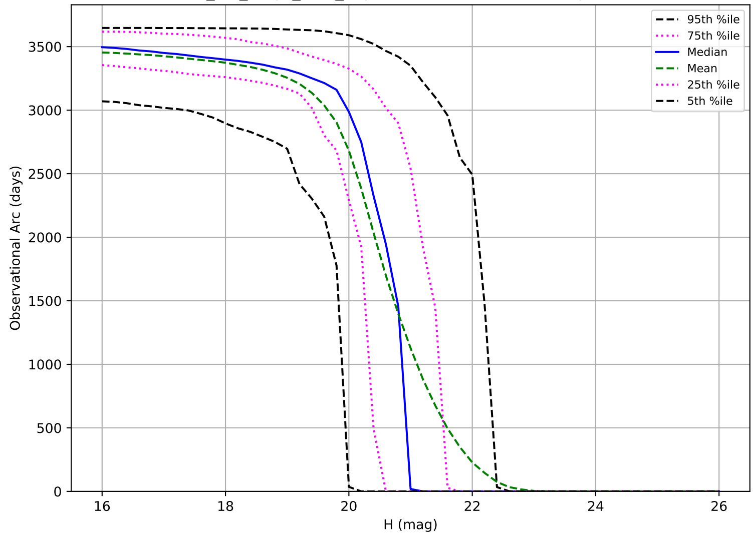
mw_roll_bulge_v3.3_10yrs: Observational Arc Length MBA
