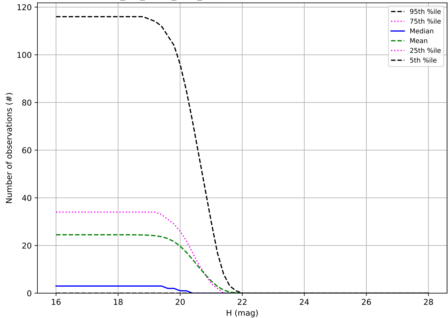
mw_roll_bulge_v3.3_10yrs: Number of observations Vatira
