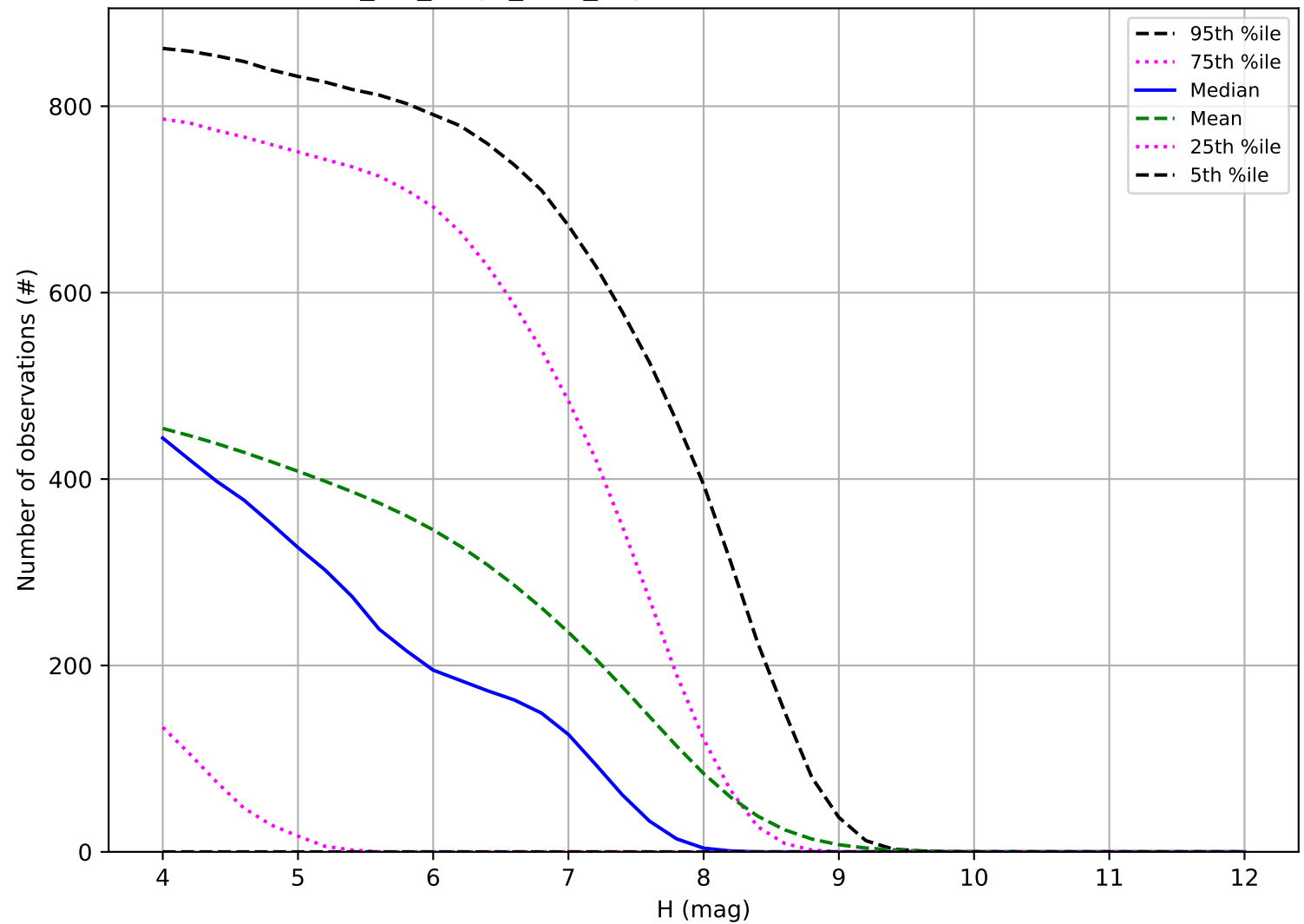
mw_roll_bulge_v3.3_10yrs: Number of observations TNO
