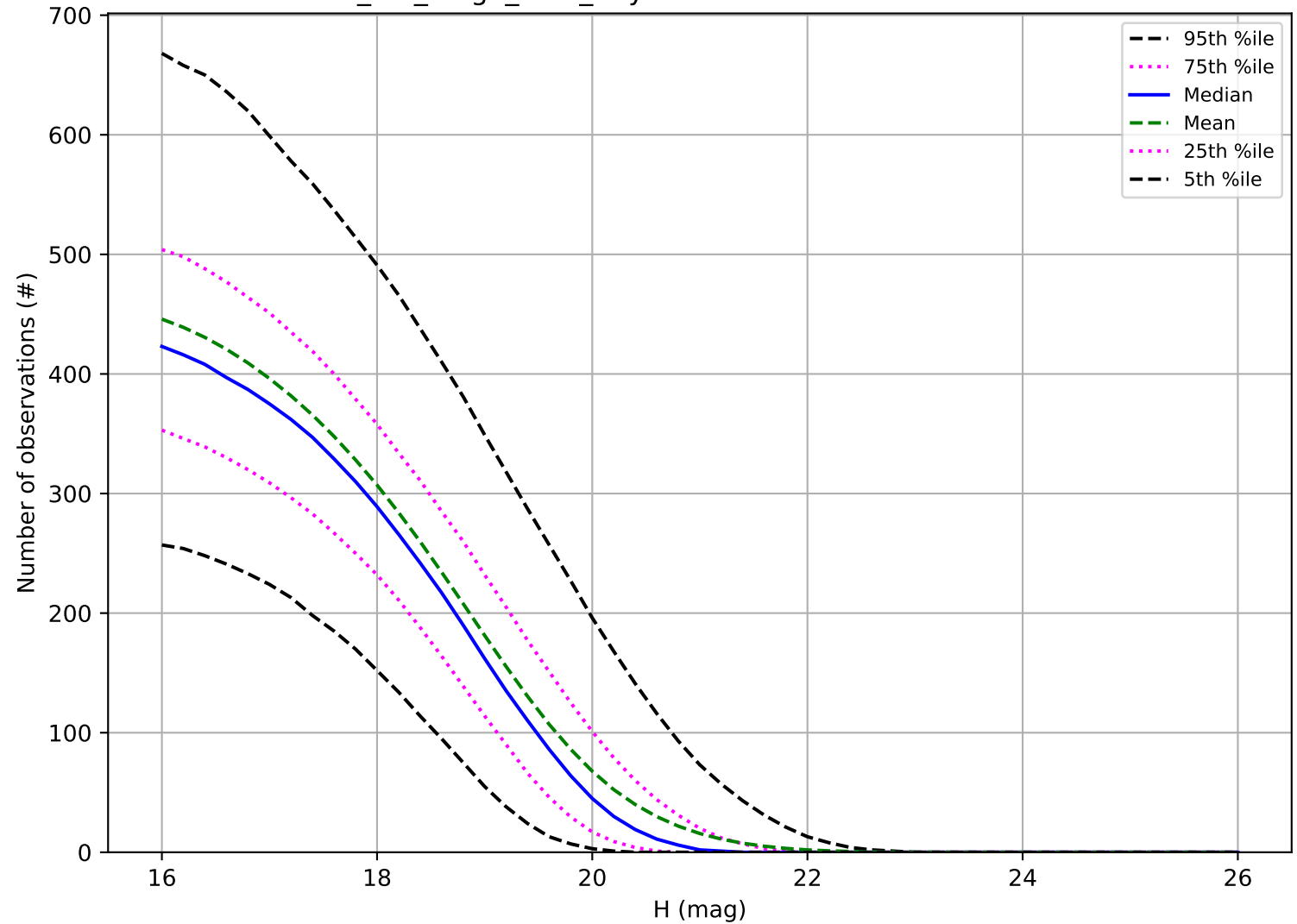
mw_roll_bulge_v3.3_10yrs: Number of observations MBA
