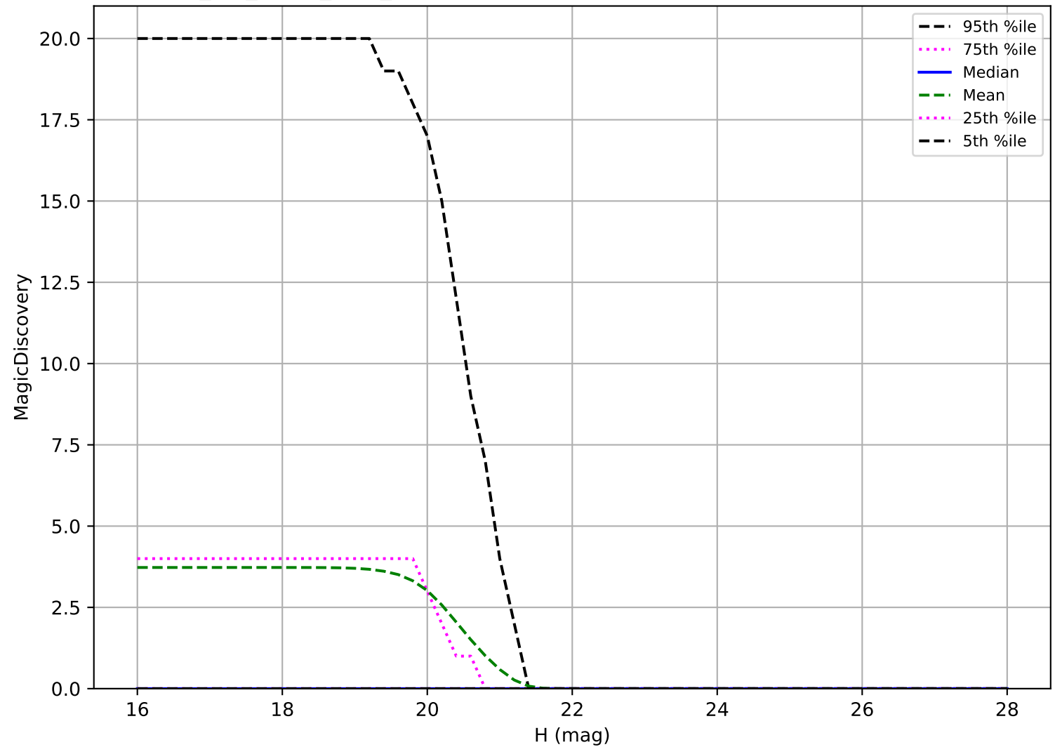
mw_roll_bulge_v3.3_10yrs: Vatira 6 detections in 60 nights detection loss
