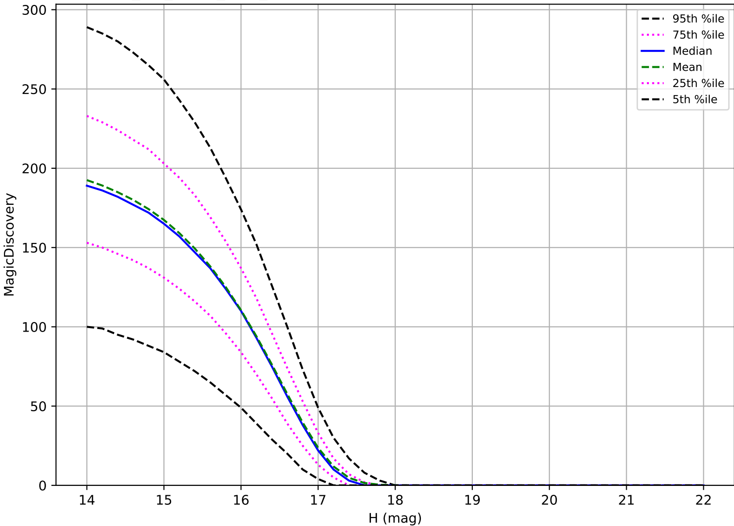
mw_roll_bulge_v3.3_10yrs: Trojan 6 detections in 60 nights detection loss
