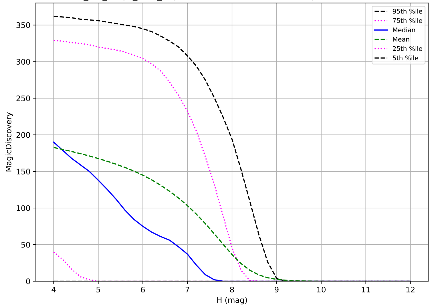
mw_roll_bulge_v3.3_10yrs: TNO 6 detections in 60 nights detection loss
