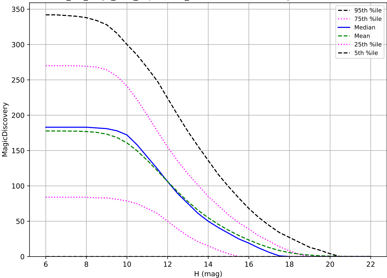
mw_roll_bulge_v3.3_10yrs: OCC_r5 6 detections in 60 nights detection loss
