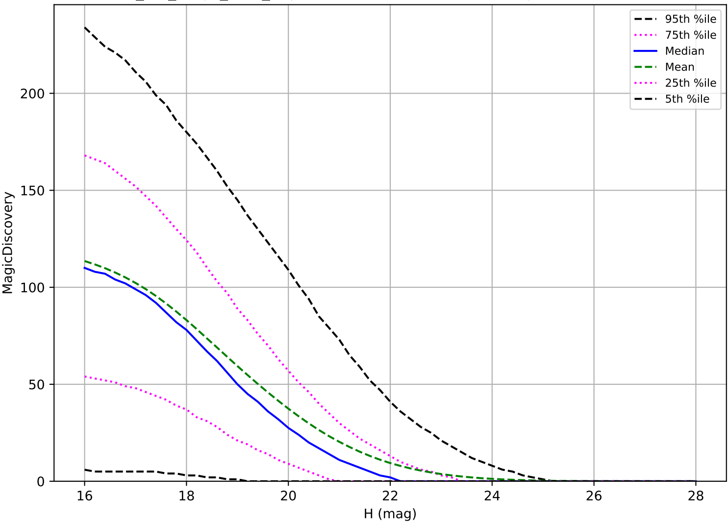
mw_roll_bulge_v3.3_10yrs: NEO 6 detections in 60 nights detection loss
