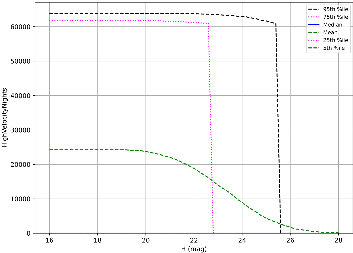
mw_roll_bulge_v3.3_10yrs: PHA High velocity pair detection loss
