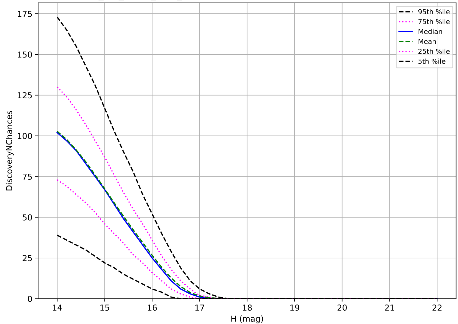
mw_roll_bulge_v3.3_10yrs: Trojan 3 pairs in 15 nights detection loss
