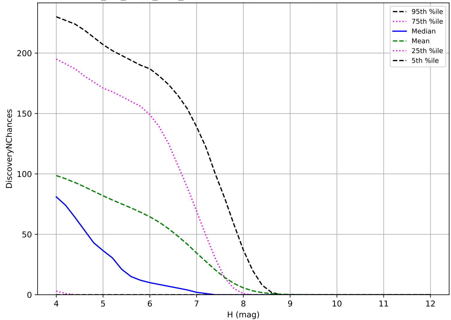
mw_roll_bulge_v3.3_10yrs: TNO 3 pairs in 15 nights detection loss
