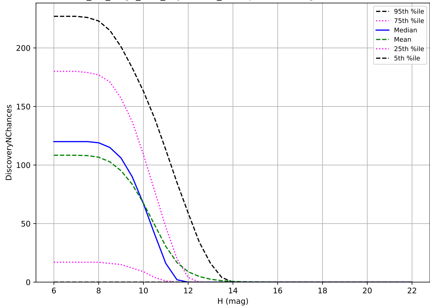
mw_roll_bulge_v3.3_10yrs: OCC_r20 3 pairs in 15 nights detection loss
