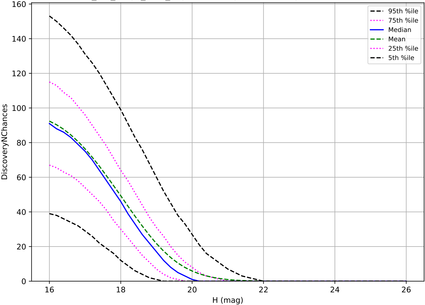
mw_roll_bulge_v3.3_10yrs: MBA 3 pairs in 15 nights detection loss
