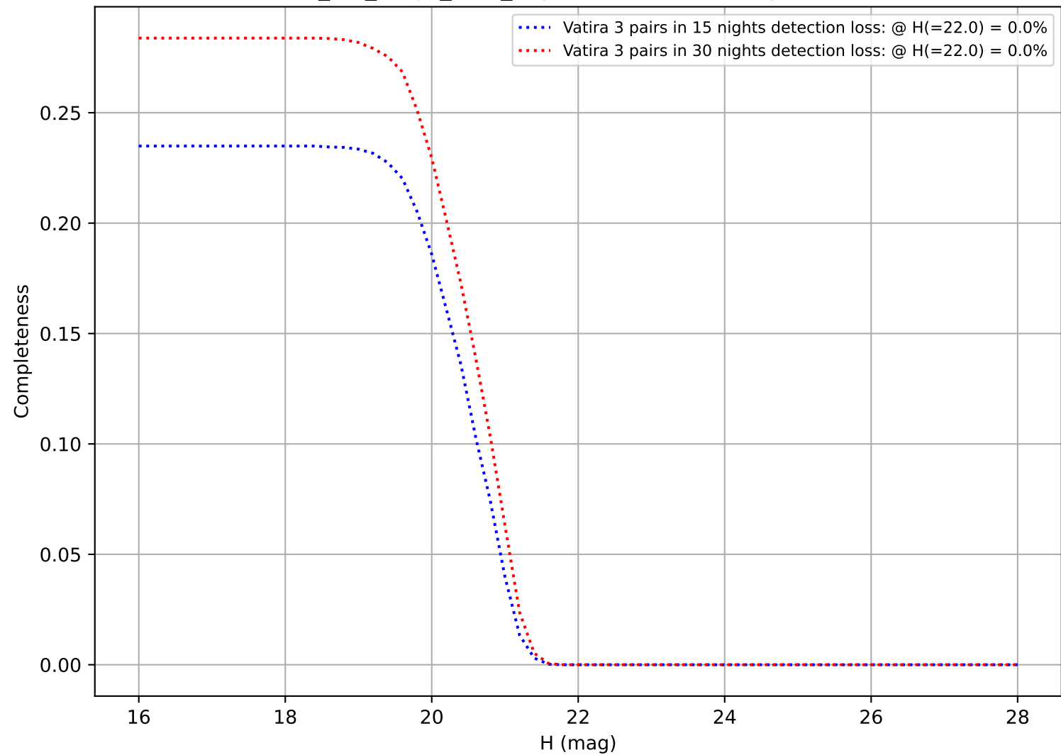
mw_roll_bulge_v3.3_10yrs: DifferentialCompleteness
