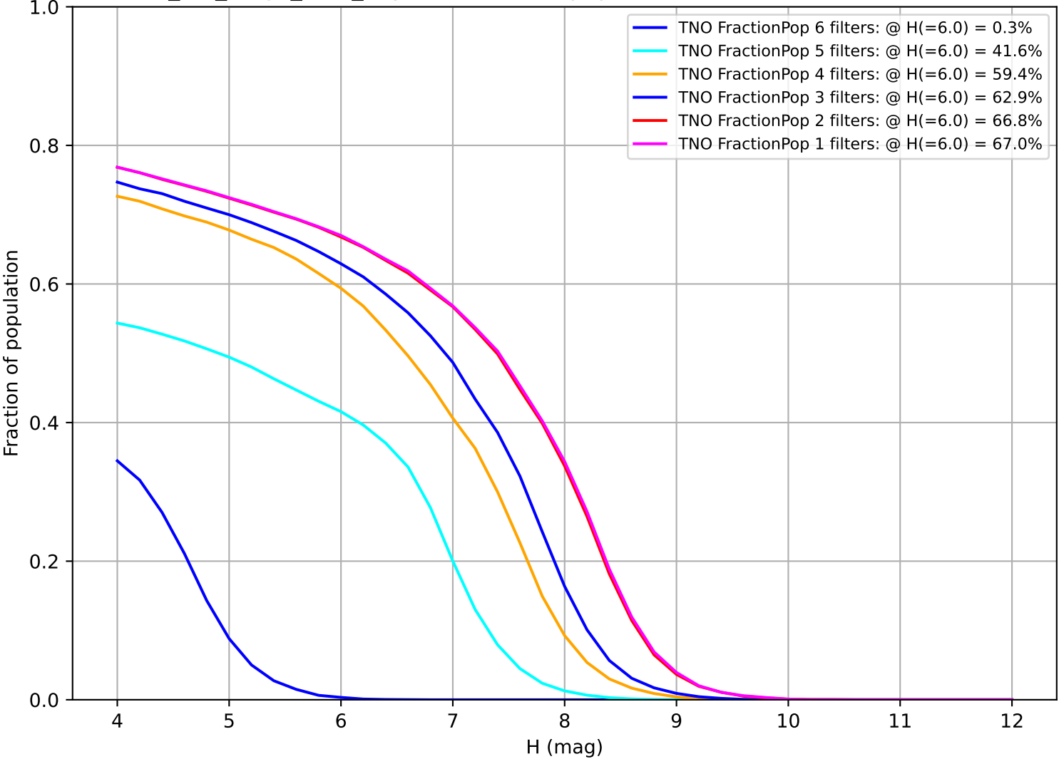
mw_roll_bulge_v3.3_10yrs: Fraction of population with colors in X filters TNO
