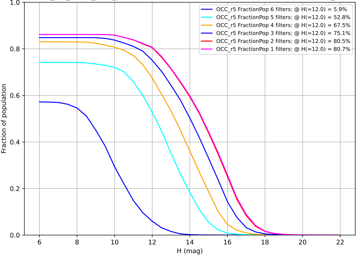
mw_roll_bulge_v3.3_10yrs: Fraction of population with colors in X filters OCC_r5
