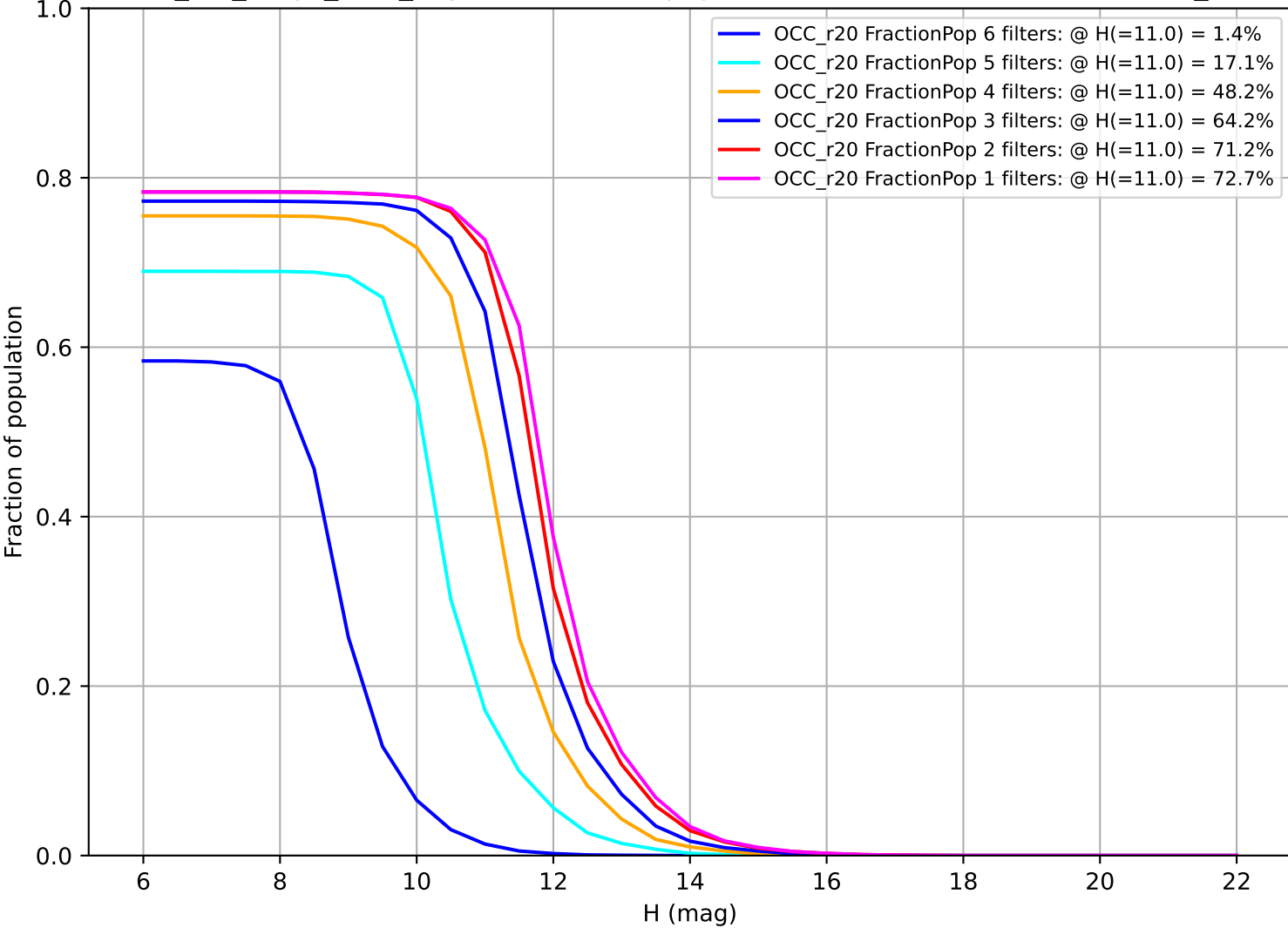
mw_roll_bulge_v3.3_10yrs: Fraction of population with colors in X filters OCC_r20
