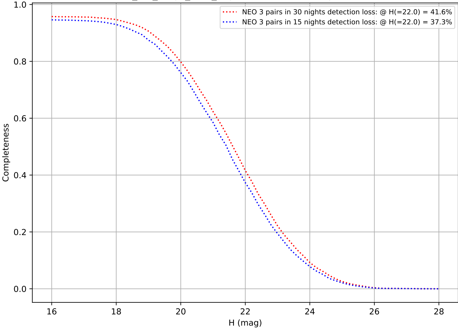
mw_roll_bulge_v3.3_10yrs: DifferentialCompleteness
