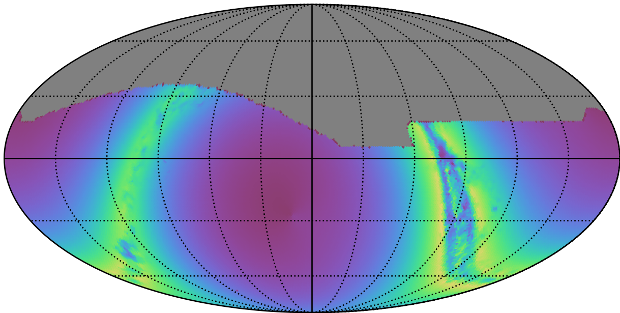
mw_roll_bulge_v3.3_10yrs : young_stars
