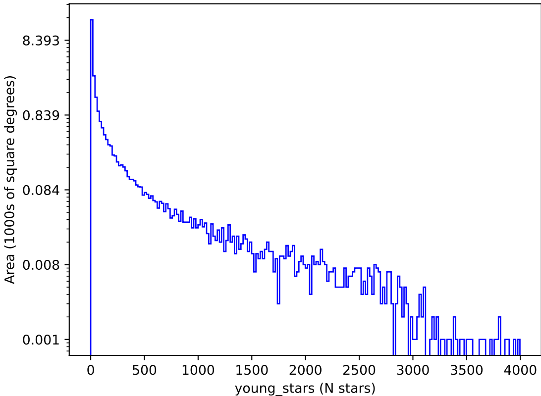
mw_roll_bulge_v3.3_10yrs : young_stars
