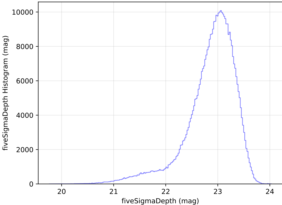
mw_roll_bulge_v3.3_10yrs z: fiveSigmaDepth Histogram
