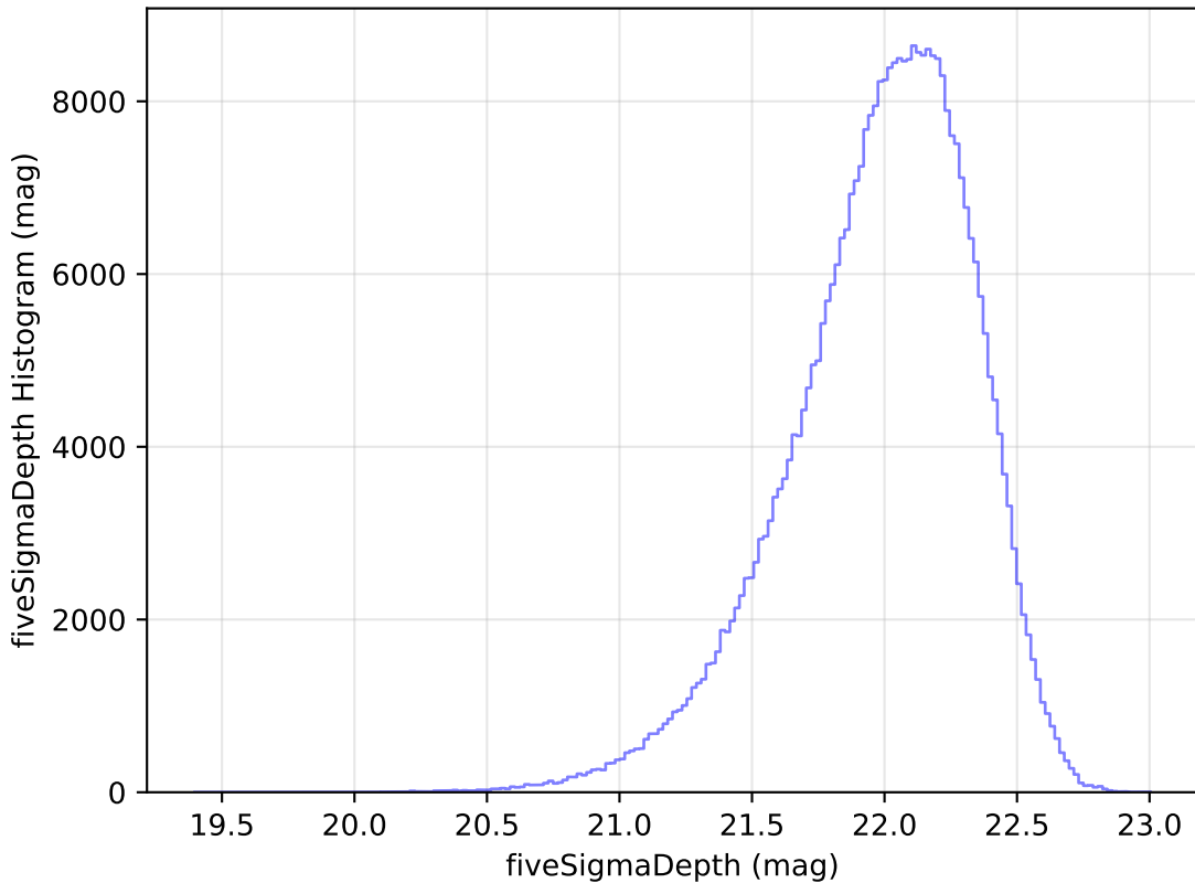
mw_roll_bulge_v3.3_10yrs y: fiveSigmaDepth Histogram
