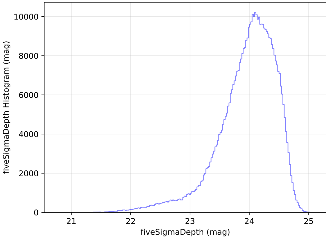
mw_roll_bulge_v3.3_10yrs r: fiveSigmaDepth Histogram
