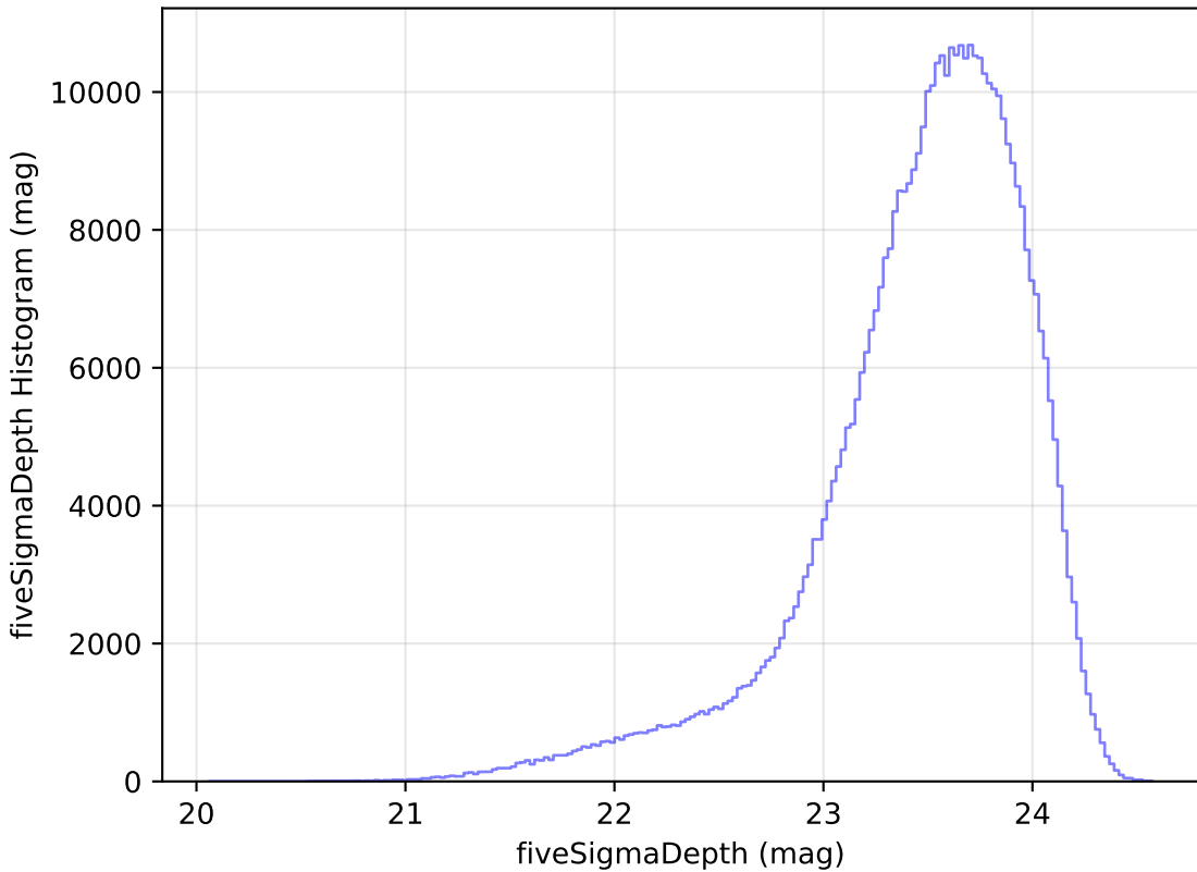
mw_roll_bulge_v3.3_10yrs i: fiveSigmaDepth Histogram
