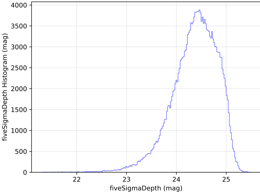
mw_roll_bulge_v3.3_10yrs g: fiveSigmaDepth Histogram
