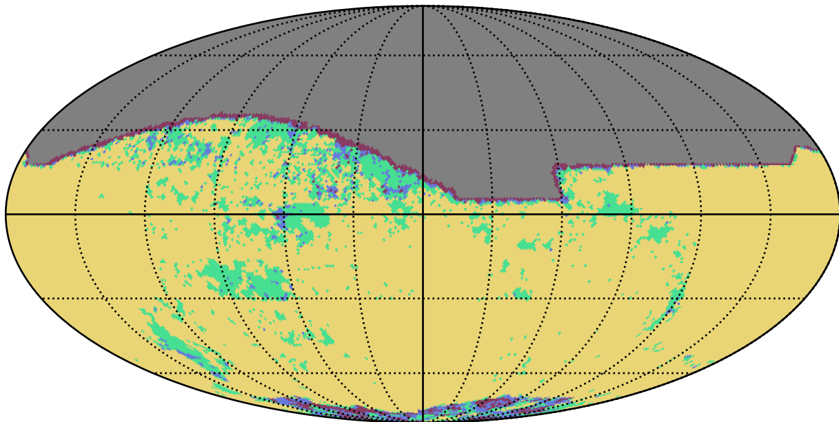
mw_roll_bulge_v3.3_10yrs z band: YearCoverage night
