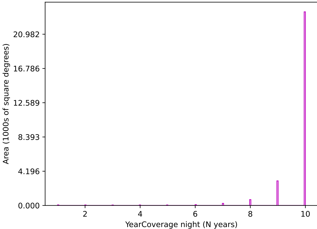
mw_roll_bulge_v3.3_10yrs z band: YearCoverage night
