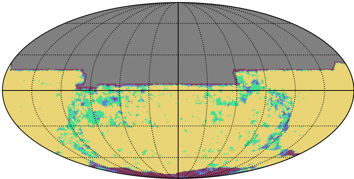
mw_roll_bulge_v3.3_10yrs y band: YearCoverage night
