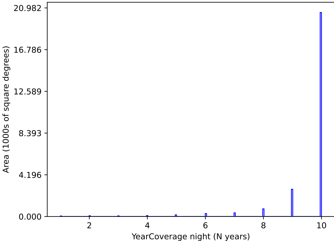
mw_roll_bulge_v3.3_10yrs y band: YearCoverage night
