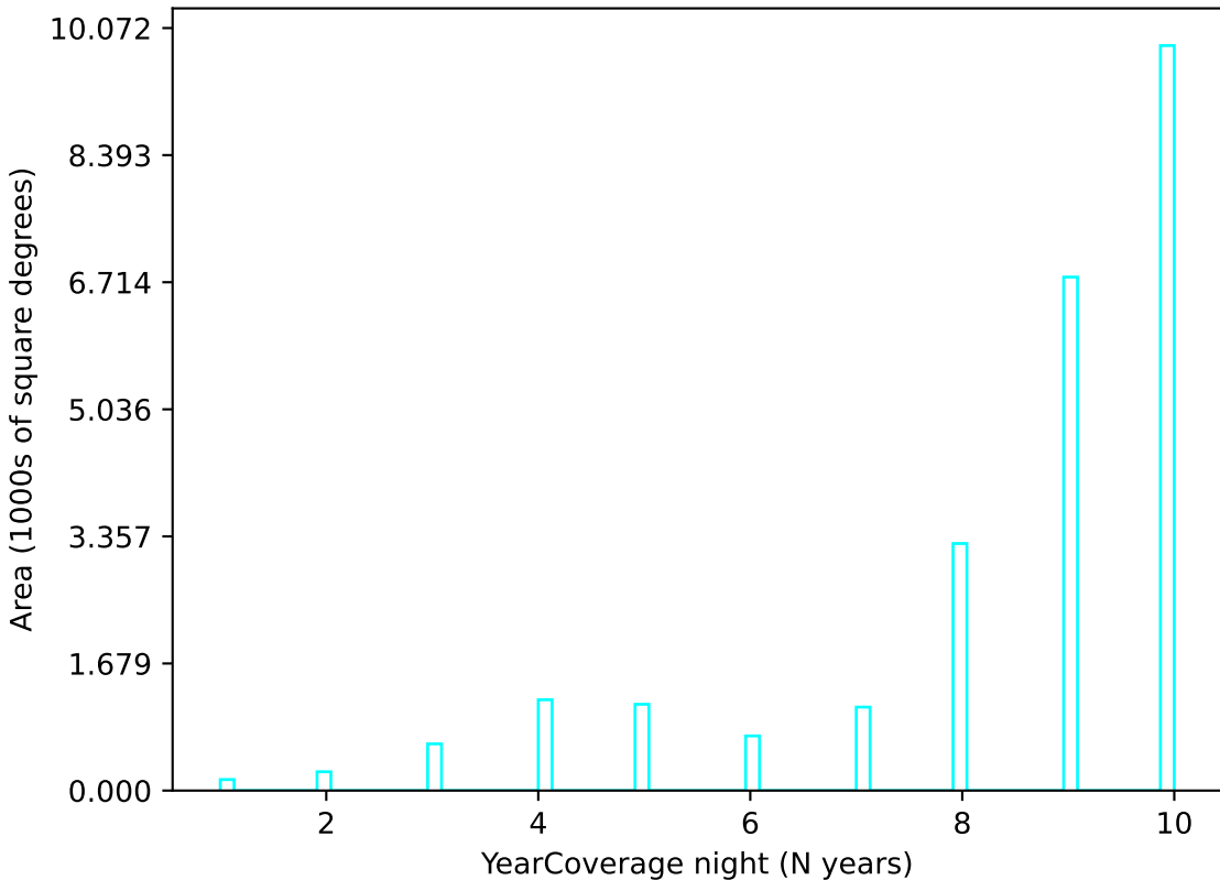
mw_roll_bulge_v3.3_10yrs u band: YearCoverage night
