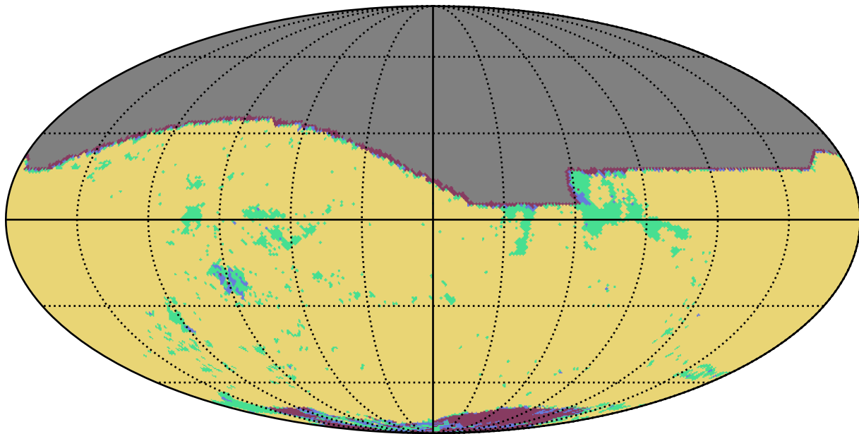
mw_roll_bulge_v3.3_10yrs r band: YearCoverage night
