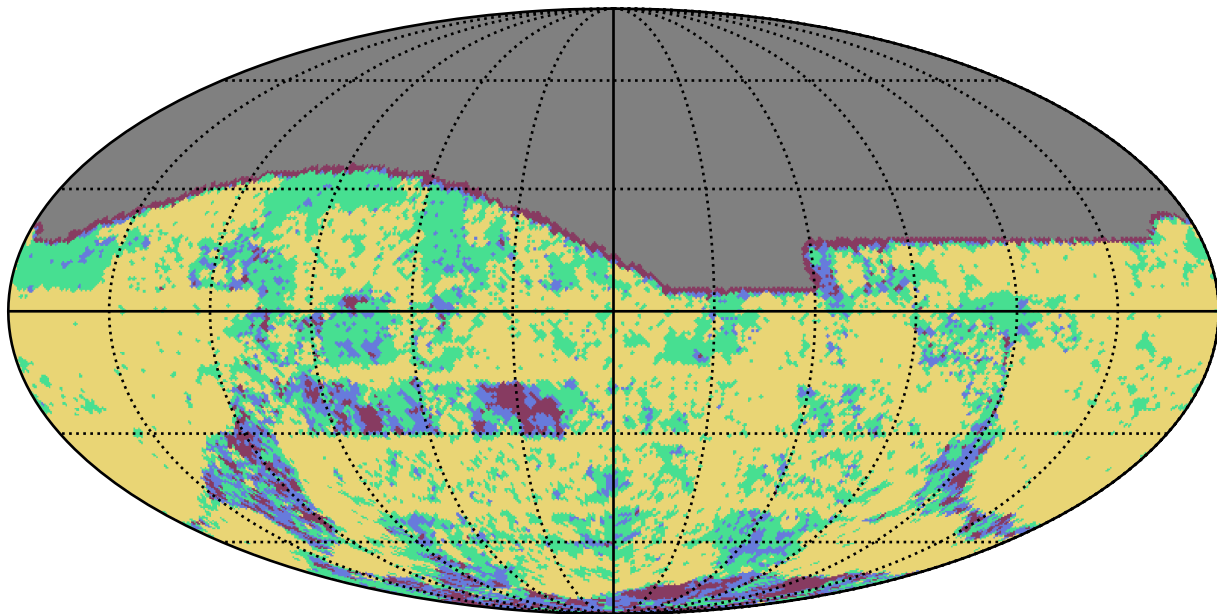
mw_roll_bulge_v3.3_10yrs g band: YearCoverage night
