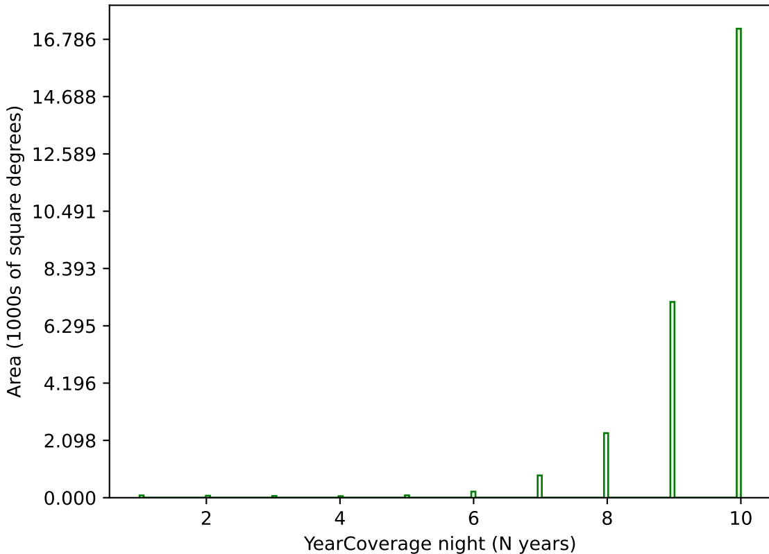
mw_roll_bulge_v3.3_10yrs g band: YearCoverage night
