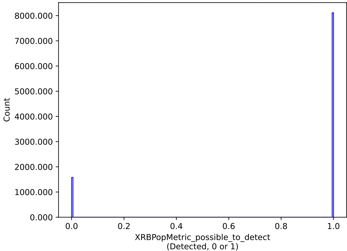
mw_roll_bulge_v3.3_10yrs : XRBPpopMetric_possible_to_detect
