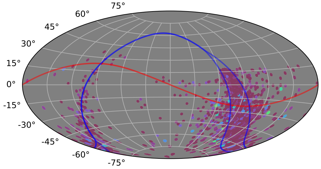
mw_roll_bulge_v3.3_10yrs : XRBPopMetric_number_of_detections
