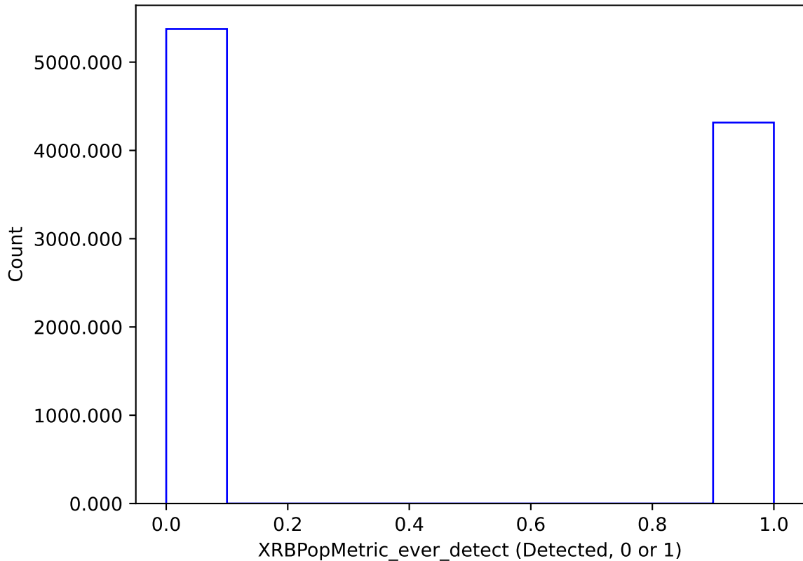
mw_roll_bulge_v3.3_10yrs : XRBPoMetric_ever_detect
